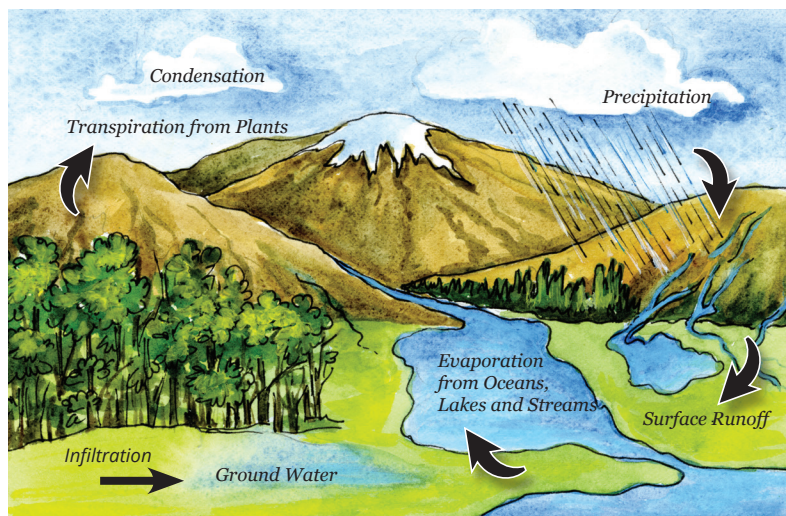
Figure 1-1: Water cycle
