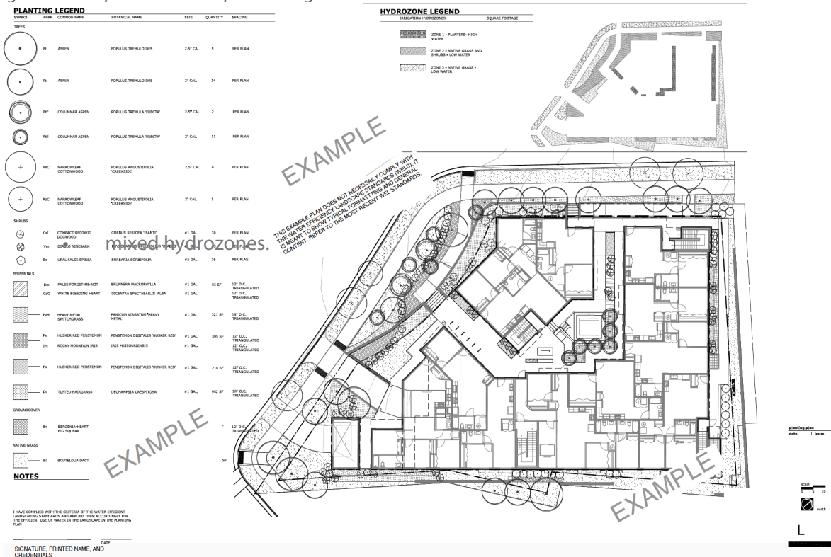
Figure 1B-2: Aspen WELS Example Planting Plan
